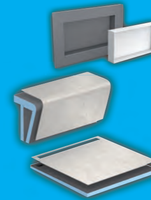
B Preformed seamless surface for the shower tray
